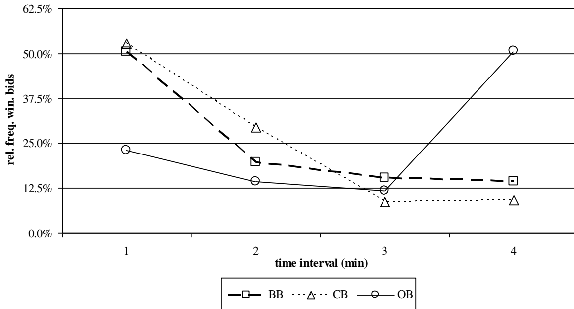
Figure 1. Share of "winning" bids per minute interval
