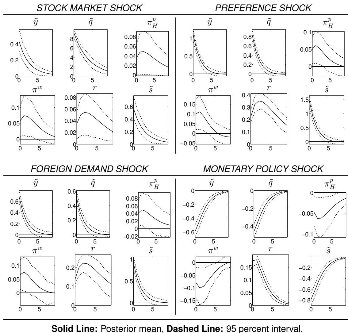
Figure 2: Bayesian Impulse Response Functions
