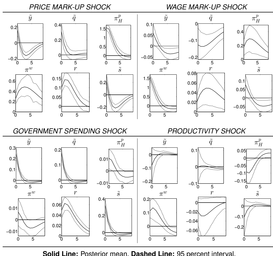
Figure 3: Bayesian Impulse Response Functions II
