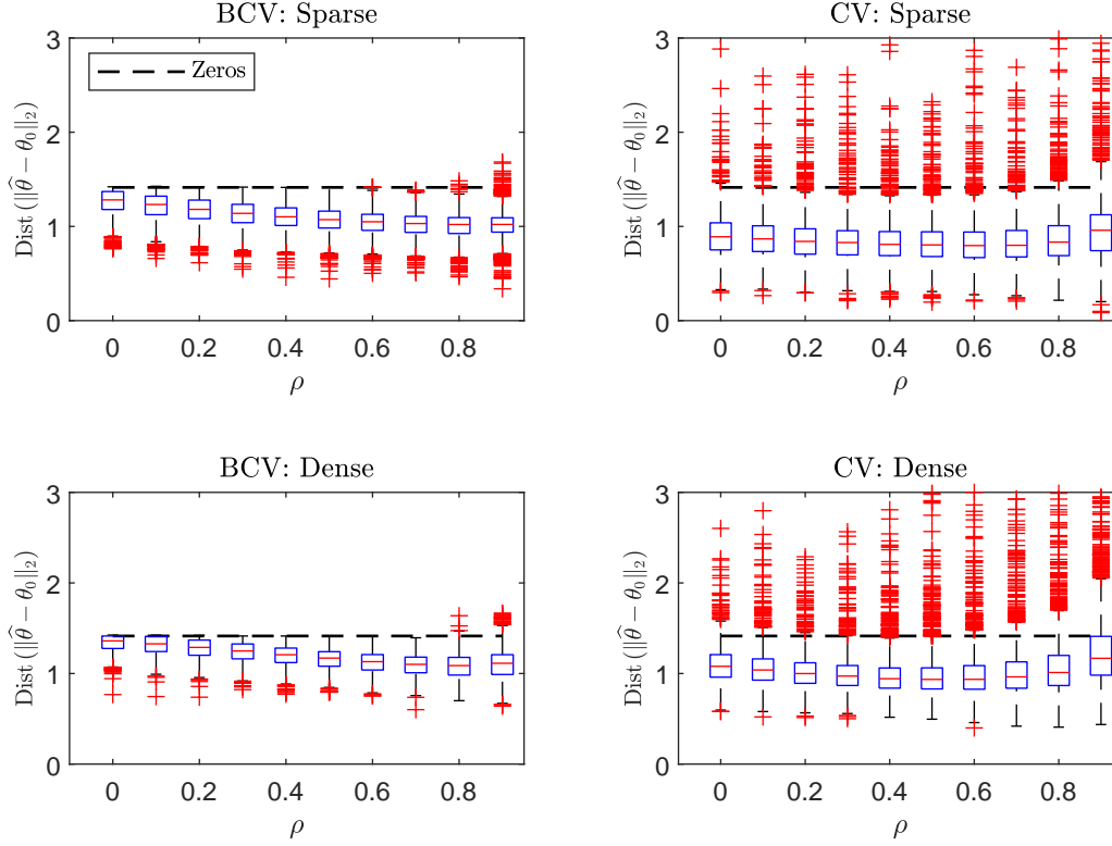
Figure 7.9: Cross-Validation and Bootstrapping after Cross-Validation ( c_0 = 1.1 ), n, p = 100 .
