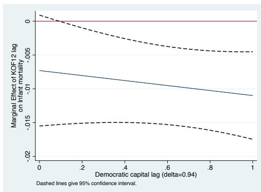
(c) Democratic capital ( \delta = 0.94 )
