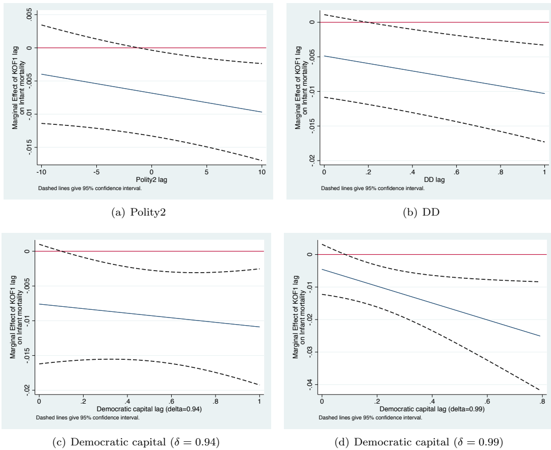
Figure 4: Marginal effects of KOF1 given democracy
