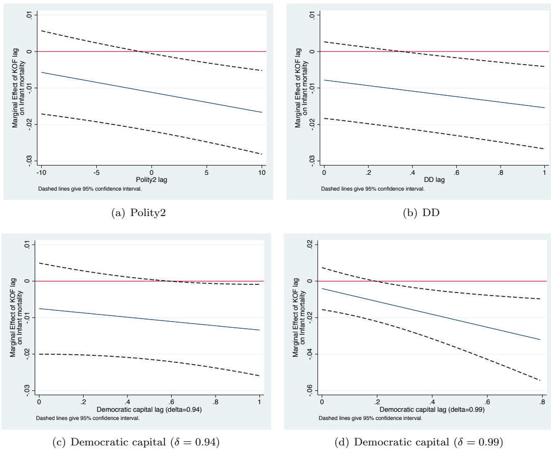
Figure 3: Marginal effects of KOF on infant mortality given democracy
