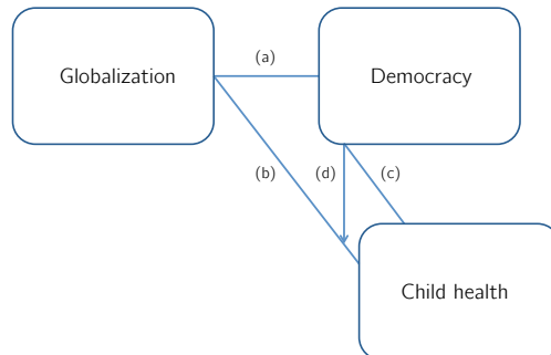
Figure 1: Globalization, democracy, and child health
