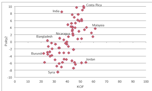
(a) KOF and Polity2
