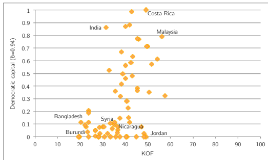
(c) KOF and Democratic capital ( \delta = 0.94 )
