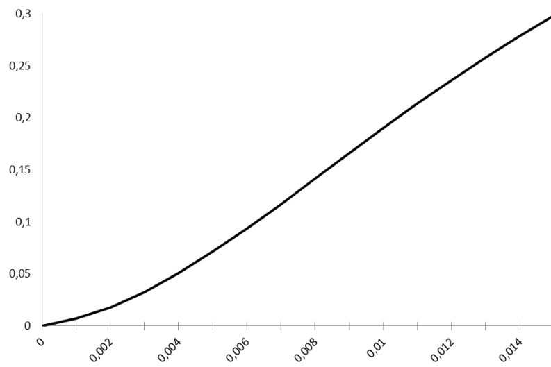
Figure 2 The “semi-analytical” asset correlation bias as a function of the exchange rate volatility of the US dollar index (USDIX) computed using equation (1) with input-parameters estimated from the actual empirical sample. All the parameters are listed in Tables 1 and 2.
