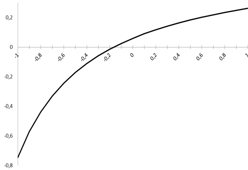
Figure 3 The “semi-analytical” asset correlation bias as a function of the asset value - exchange rate correlation for the US dollar index (USDIX) computed using equation (1) with input-parameters estimated from the actual empirical sample. All the parameters are listed in Tables 1 and 2.
