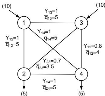
Figure 1: The basic structure and parameters of the 4-node network. Y_{ij} corresponds to the admittance value of the line between i and j , while \bar{q}_{ij} denotes the value of the maximal possible energy transfer on the corresponding line (power transmission capacity). The numbers in parentheses at the nodes correspond to maximal generating capacity and desired consumption.
