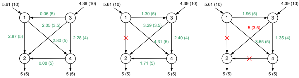
Figure 2: Basic (safe) operation of the 4 node network without failures, flows without rescheduling in the case of the failure of line 1-2, and in the case of the failure of line 1-2 and 2-4: The first failure does not lead to line overload, but without rescheduling the second failure causes the overload of line 2-3.
