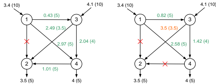
Figure 3: Rescheduling of the network after the failure of line 1-2: The second failure of line 2-4 does not overload the remaining lines. Line 2-3 operating on the edge of his capacity shows, that the rescheduling of generators and the curtailment of loads was justified.
