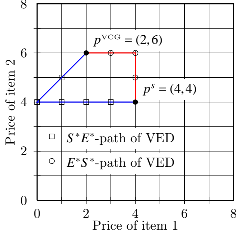
Figure 1: The E^*S^* -path and the S^*E^* -path of the Vickrey-English-Dutch auction for starting prices p^s = (4, 4) .
