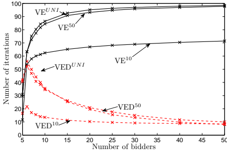
Figure 2: The mean number of iterations for the E^*S^* -path of VED and the Vickrey-English auction (VE) for the different problem sizes and distributions.
