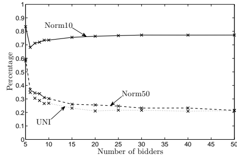
Figure 5: Percentage fewer iterations required for the E^*S^* -path of VED compared to the Vickrey-Dutch auction given that the E^*S^* -path of VED is faster than the Vickrey-Dutch auction.
