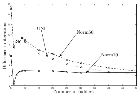
Figure 6: Average difference in iterations between the E^*S^* -path of VED and Greedy VED for the different problem sizes and distributions.
