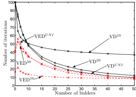
Figure 3: The mean number of iterations for the E^*S^* -path of VED and the Vickrey-Dutch auction (VD) for the different problem sizes and distributions.
