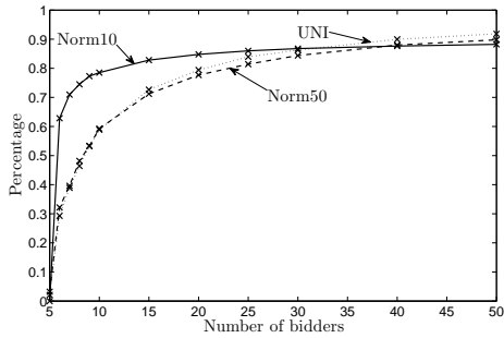
Figure 4: Percentage fewer iterations required for the E^*S^* -path of VED compared to the Vickrey-English auction given that the E^*S^* -path of VED is faster than the Vickrey-English auction.
