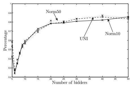
Figure 7: Percentage of the problems where the required iterations for Greedy VED equals the required iterations for The Shortest Path.
