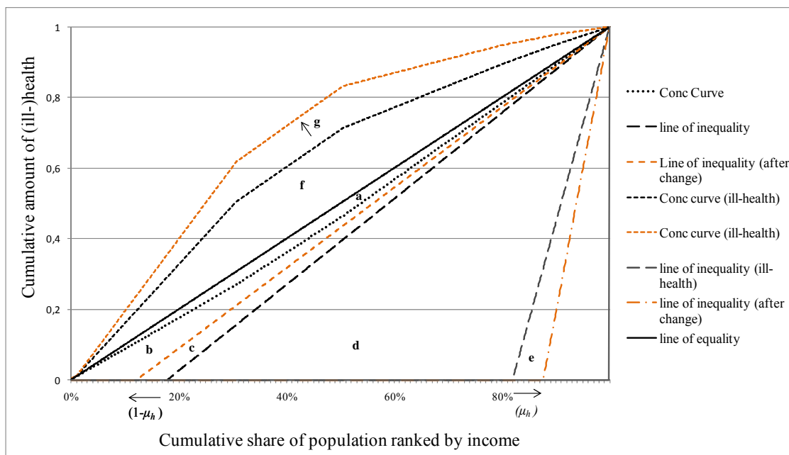
Figure 2: The response of W to equiproportional changes
