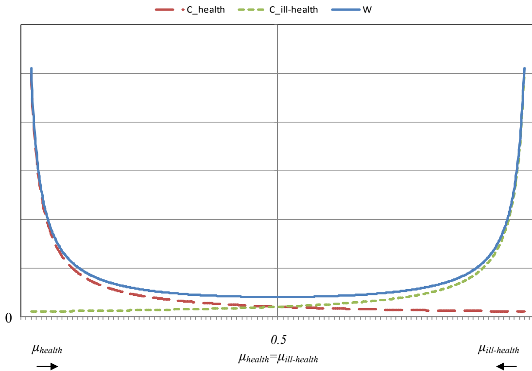
Figure 5: Thresholds of latent variables
