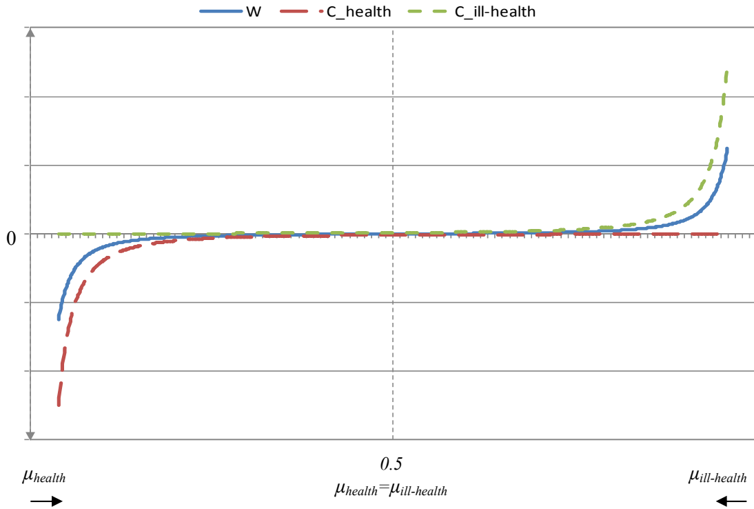
Figure 3: Marginal response ( \partial f(H)/\partial \mu_h ) of W , C(\text{health}) and C(\text{ill-health})
