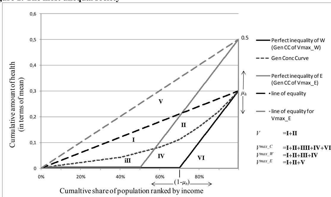
Figure 1: The most unequal society
