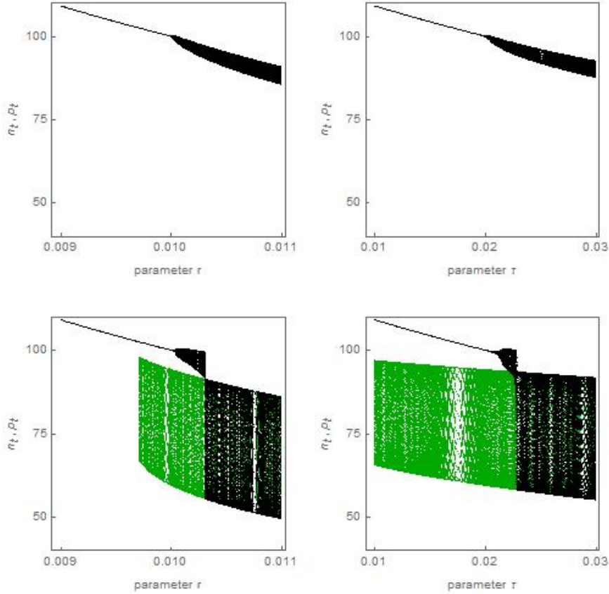
Figure 7: Effects of the discount rate on the stability and out-of-equilibrium behavior of the model. The top left and top right panels show bifurcation diagrams of n_t = p_t (black) against parameters r and \tau , respectively. All other parameters correspond to our base parameter setting. The bottom panels show the same, except that \kappa = 0.4 and m = 0.5 . Green shading represents a co-existing attractor, resulting from different initial conditions.
