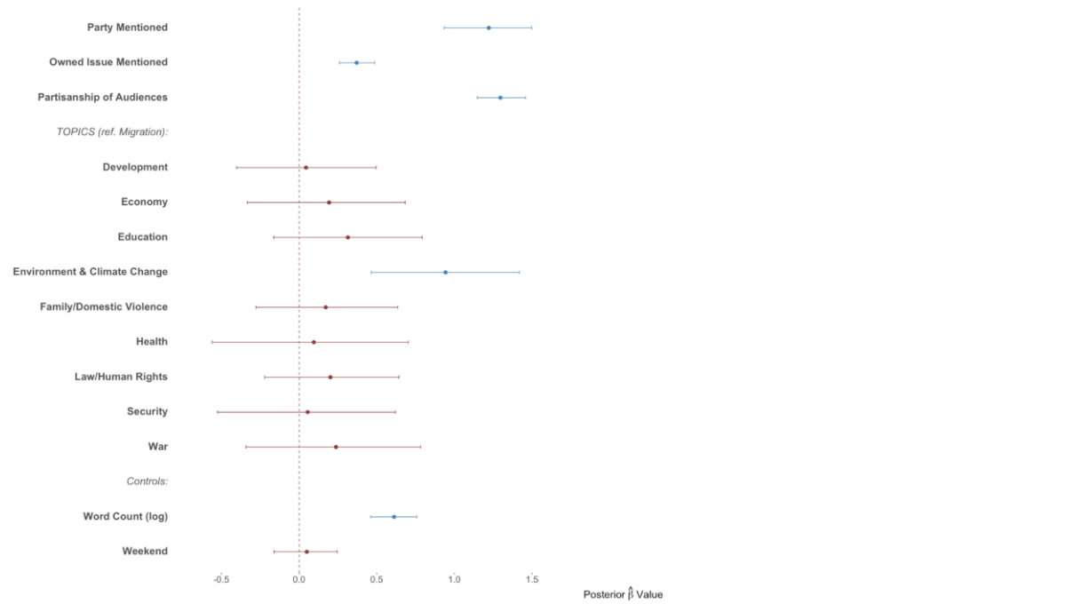
Figure A3. Posterior Distribution of Model Parameters. Spanish Cases Only.
