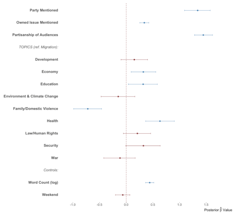
Figure A4. Posterior Distribution of Model Parameters. UK Cases Only.
