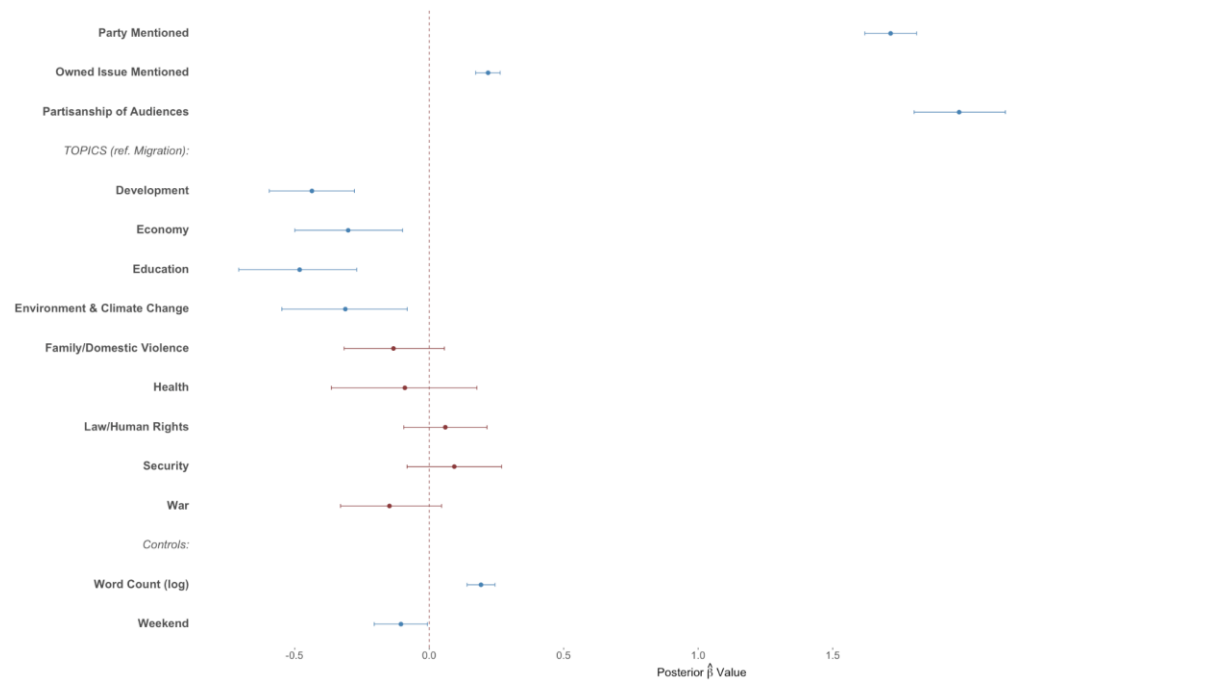
Figure A2. Posterior Distribution of Model Parameters. German Cases Only.
