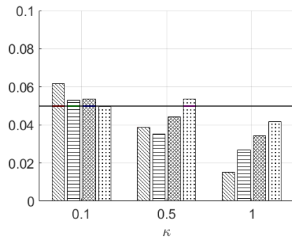
(c) \mathbb{H}_0, K_1 = 4, p = 1
