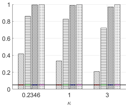
(j) \mathbb{H}_0 : \beta(1) = \beta(2) , \rho = 0.5, p = 12
