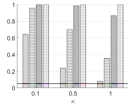
(i) \mathbb{H}_1, K_1 = 4, p = 1
