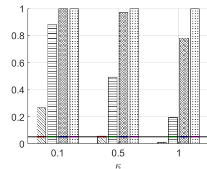
(l) \mathbb{H}_1, K_1 = 4, p = 12
