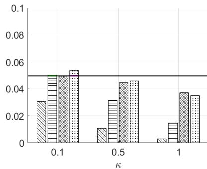
(f) \mathbb{H}_0, K_1 = 4, p = 12
