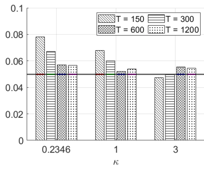
(a) \mathbb{H}_0 : \beta(1) = \beta(2) , \rho = 0, p = 1
