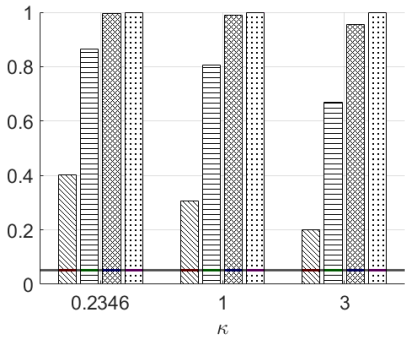
(g) \mathbb{H}_0 : \beta(1) = \beta(2) , \rho = 0, p = 12
