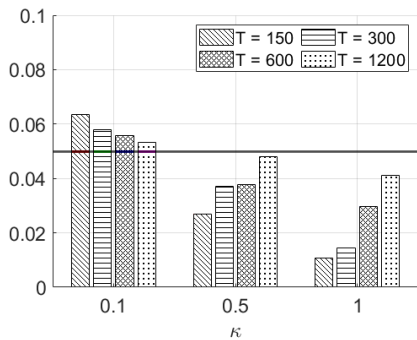
(a) \mathbb{H}_0, K_1 = 2, p = 1
