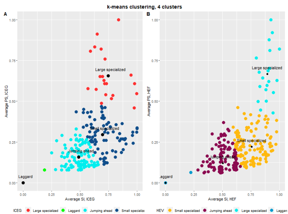
Figure 11: k-mean clustering, 4 clusters
