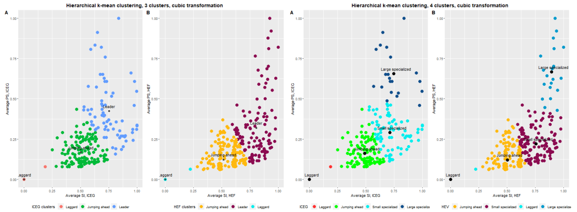
Figure 14: Hierarchical K-Means Clustering
