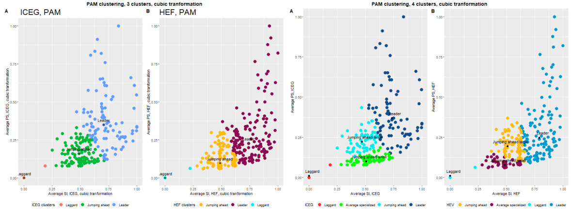
Figure 13: PAM clustering
