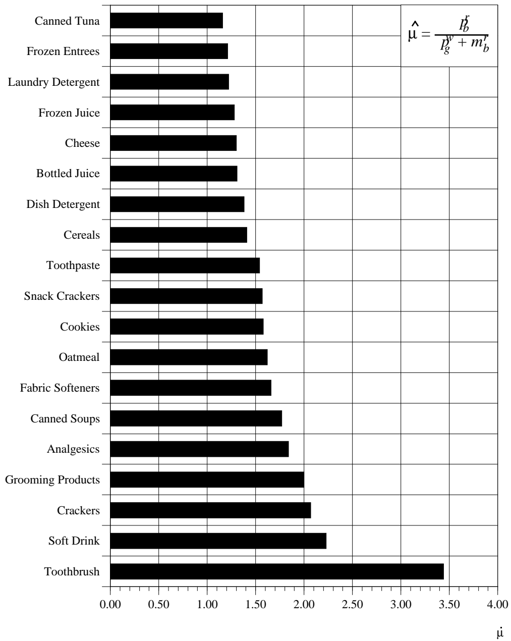
Figure 1. Markup Ratio for Branded Products: "Preferred" Lower Bound (Measure a)
