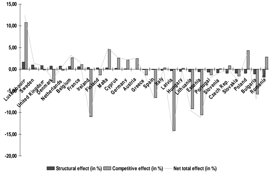
Figure 1. Dynamic shift-share
