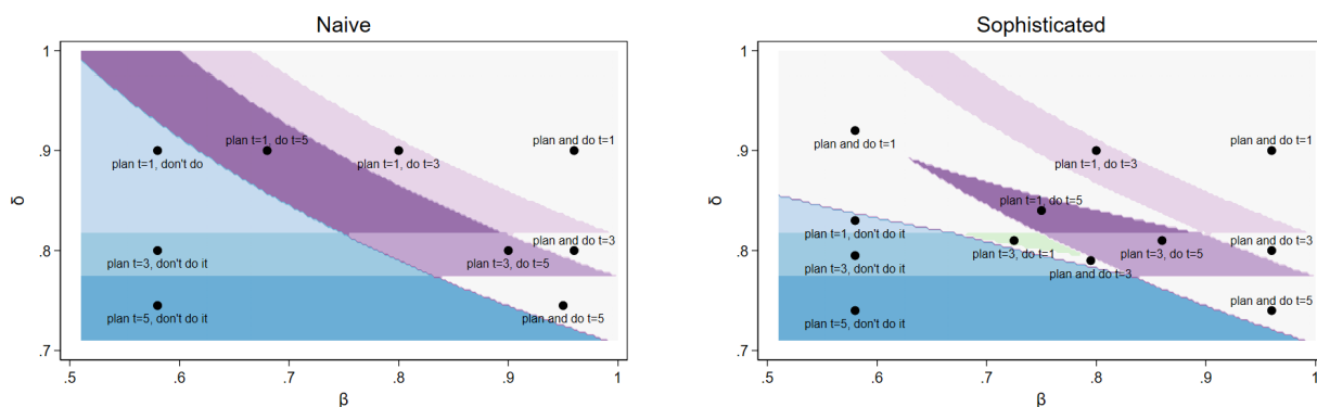
Figure 2: Model Implied Planned and Actual Behavior for Different Levels of \beta and \delta
