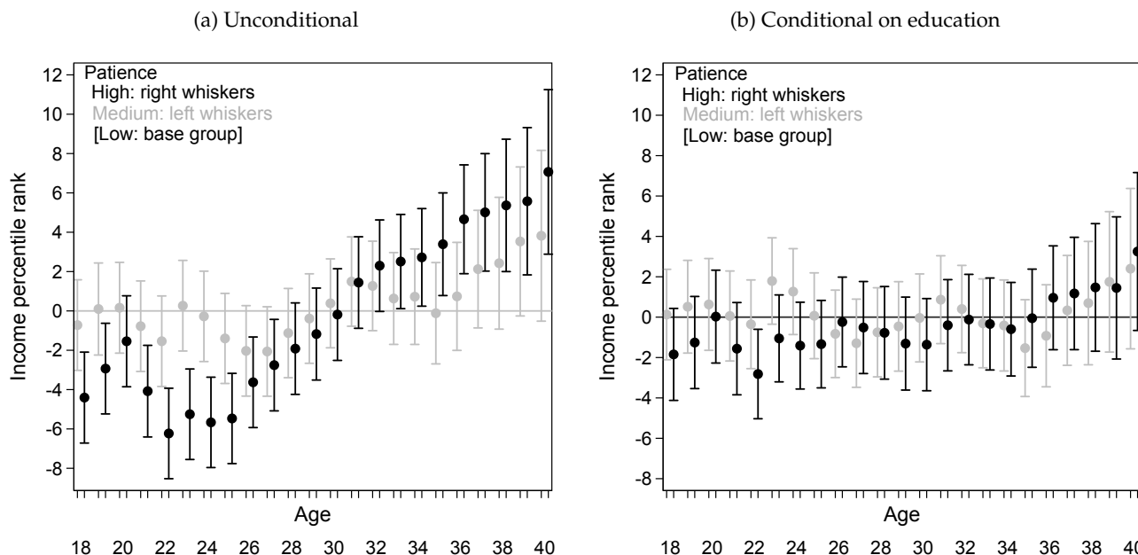
Figure 5: Relationship between discounting behavior and income over the life cycle
