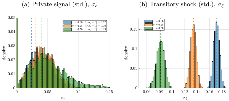
Figure C.1: Bootstrap, CEQ Model.
