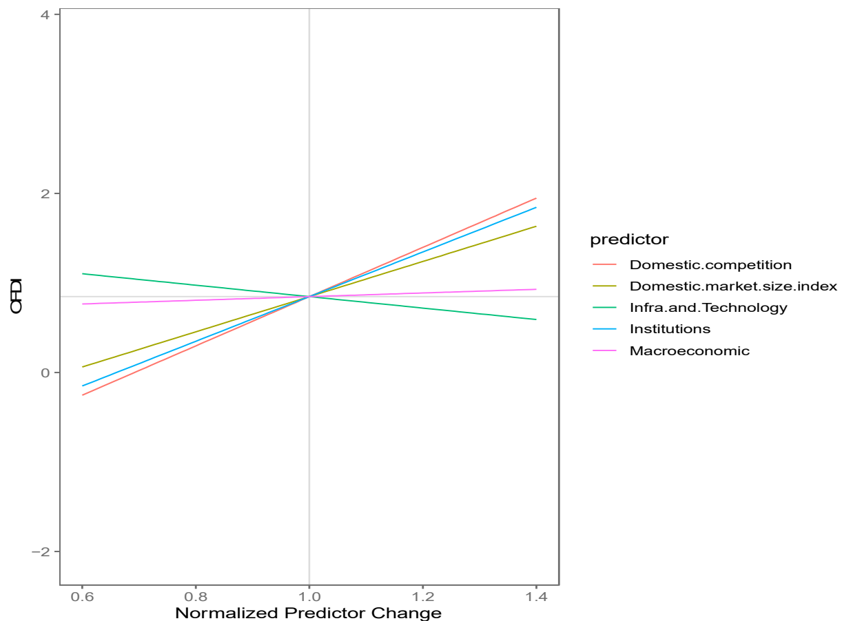
Figure 6. Sensitivity analysis for model (2) with a 90% confidence interval constructed for each predictor.
