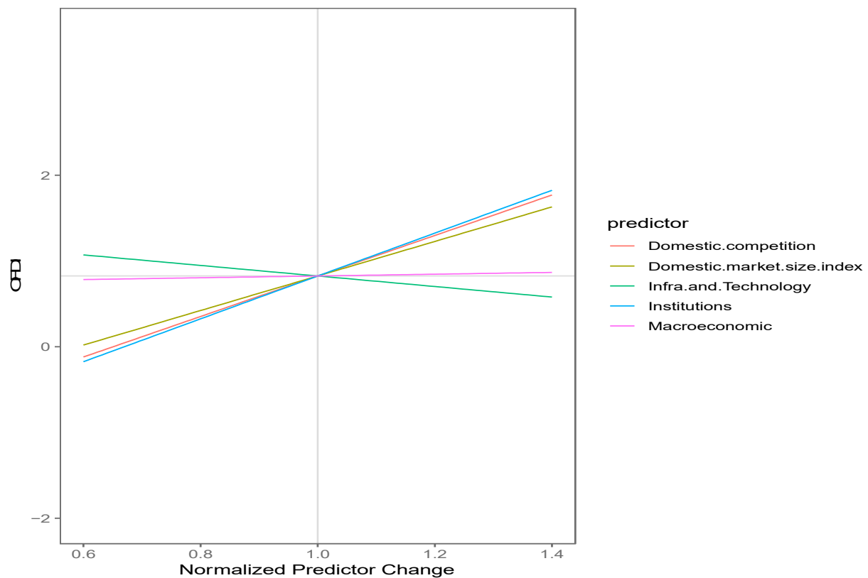
Figure 5. Sensitivity analysis for model (1) with a 90% confidence interval constructed for each predictor.
