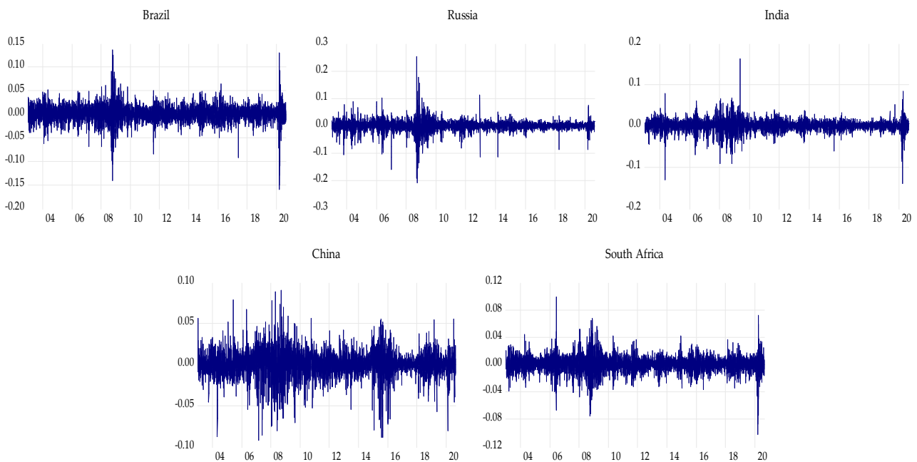
Figure 1. Daily returns series of the BRICS markets.
