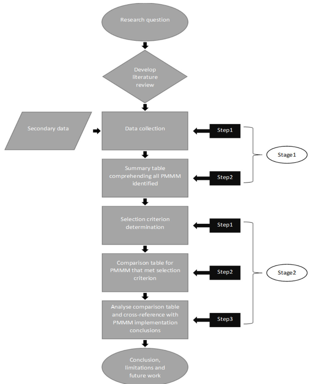
Figure 1. Methodology flowchart.
