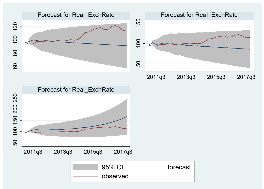
Figure 2. US—VEC-Model Forecasting.
