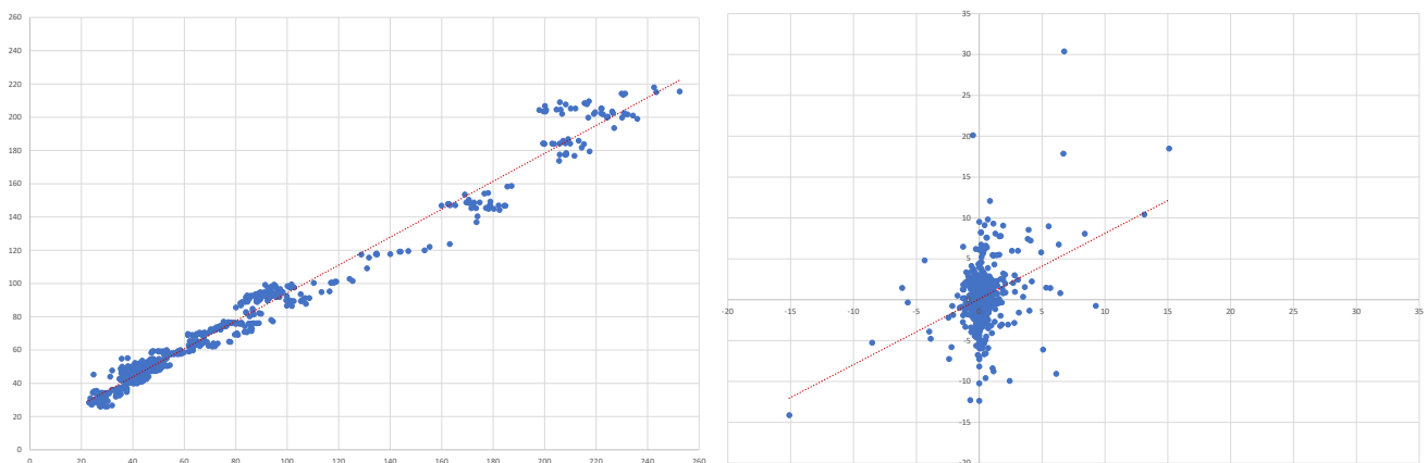
Figure A1. Adidas. Individual time series regressions using three price series on Adidas: future prices (FP), target prices (TP), and capitalised prices (CP) forecasts. On the left-hand-side are images of level regressions and on the right-hand-side are the regressions in differences.
