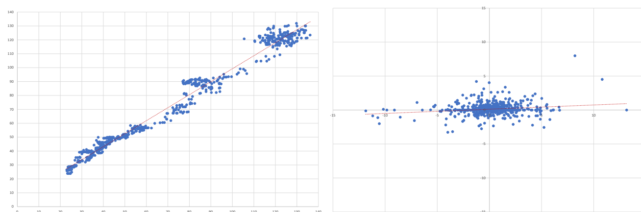
Figure A4. Essilor. Individual time series regressions using three price series on Essilor: future prices (FP), target prices (TP), and capitalised prices (CP) forecasts. On the left-hand-side are images of level regressions and on the right-hand-side are regressions in differences.
