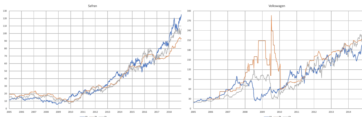
Figure 1. Comparison of target prices (TP) and capitalised prices (CP) with actual future prices (FP). Target prices (TP: orange lines) and capitalised prices (CP: grey lines) forecast for the indicated date t , jointly with actually observed future prices (FP: blue lines) at t , for the 8 best performing companies over the 15-year period of our sample: Adidas, Anheuser, ASML, Essilor, Fresenius, Inditex, Safran, Volkswagen.
