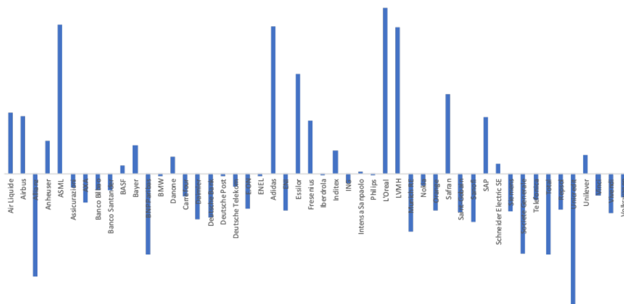
Figure 3. Company fixed effects.
