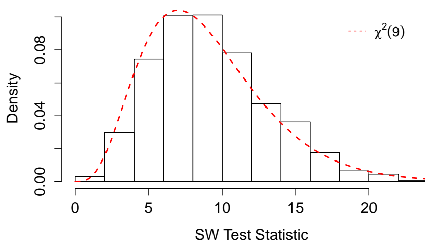
Figure 2. The empirical vs. asymptotic sampling distribution of SW by 1000 data cloning.
