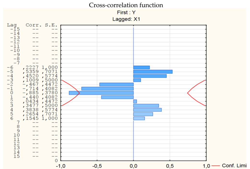
Figure 3. Cross-correlation function for GRP and GVA of the science-intensive production of the Russian Arctic zone (calculated by the authors).
