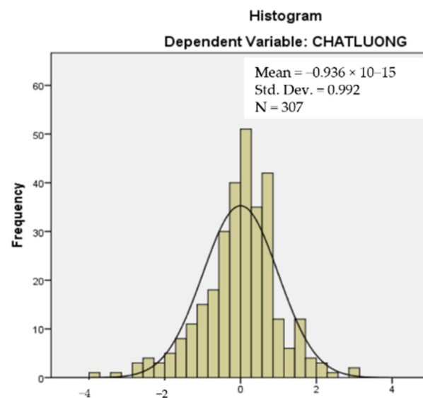
Figure 3. Regression standardized residual.
