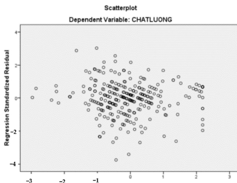
Figure 5. Regression standardized predicted value.
