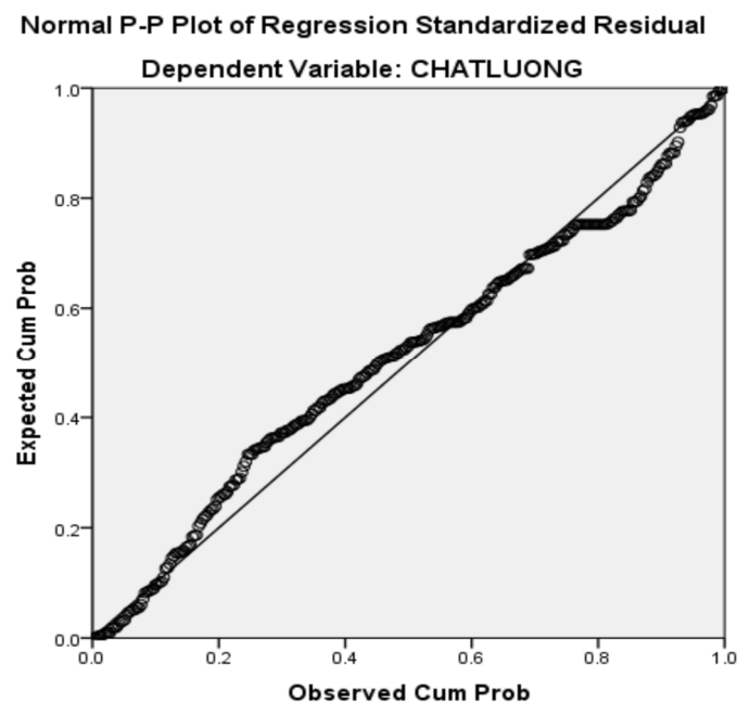
Figure 4. Normal P–P plot of regression standardized residual.
