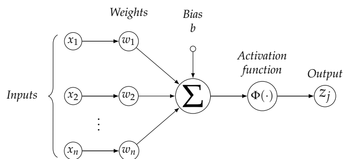
Figure 1. Representation of a node with n input features.
