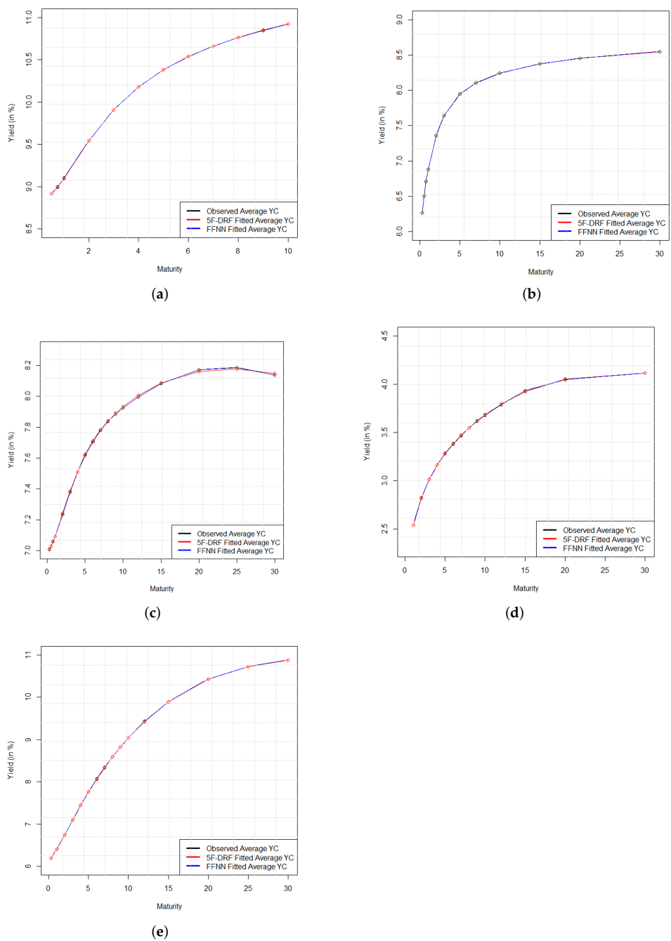
Figure 4. Average observable yield curve against average yield curves generated by the 5F-DRF (red) and FFNN (blue) models in the BRICS market. From top to bottom and from left to right, (a) is associated to Brazil, (b) to Russia, (c) to India, (d) to China, (e) to South Africa.
