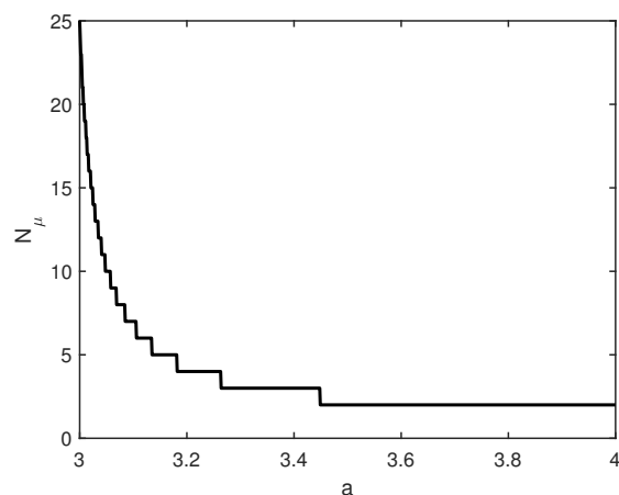
Figure 4. Minimum number of bonds w.r.t. force of mean reversion ( a ).
