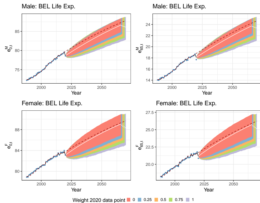
Figure 10. Estimated and projected period life expectancies \hat{e}_{x,t} for Belgium. Male ( top ) and female ( bottom ) data, ages 0 ( left ) and 65 ( right ), calibration period 1988–2020, projection period 2021–2070, method of Section 5.1. We show the 0.5%, median (white lines) and 99.5% quantile (fan charts), based on 10,000 simulations, across each weighting scenario. The dark red, dashed line shows the 50% quantile originating from the original IA|BE 2020 model. The blue dots and black line represent the observed and fitted period life expectancies, respectively.
