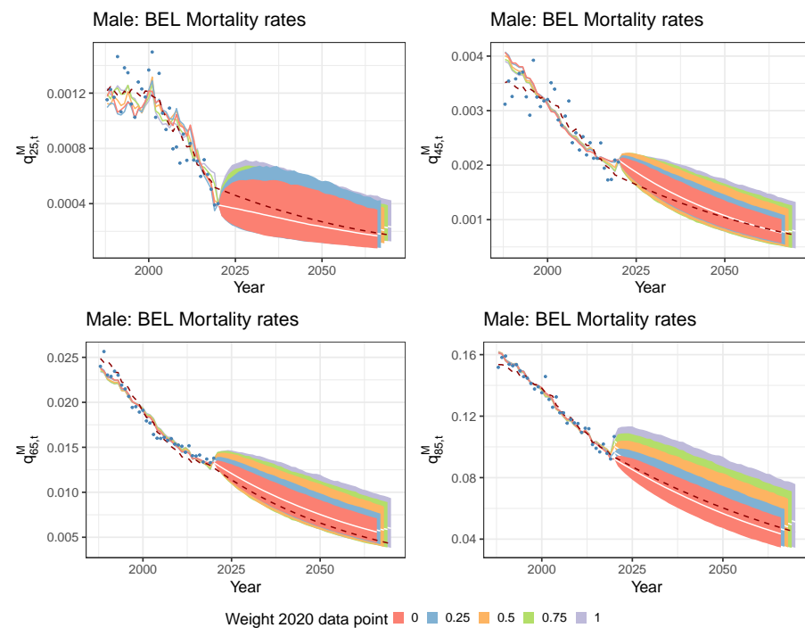
Figure 14. Estimated and projected Belgian mortality rates \hat{q}_{x,t} . Male data, ages 25, 45 ( top ) and 65, 85 ( bottom ), calibration period 1988–2020, projection period 2021–2070, method of Section 5.2. We show the 0.5%, median (white lines) and 99.5% quantile (fan charts), based on 10,000 simulations across each weighting scenario. The blue dots and the coloured, solid lines represent the observed and fitted mortality rates, respectively. The dark red, dashed line shows the calibrated mortality rates and the median quantile of simulations in the original IA|BE 2020 model.
