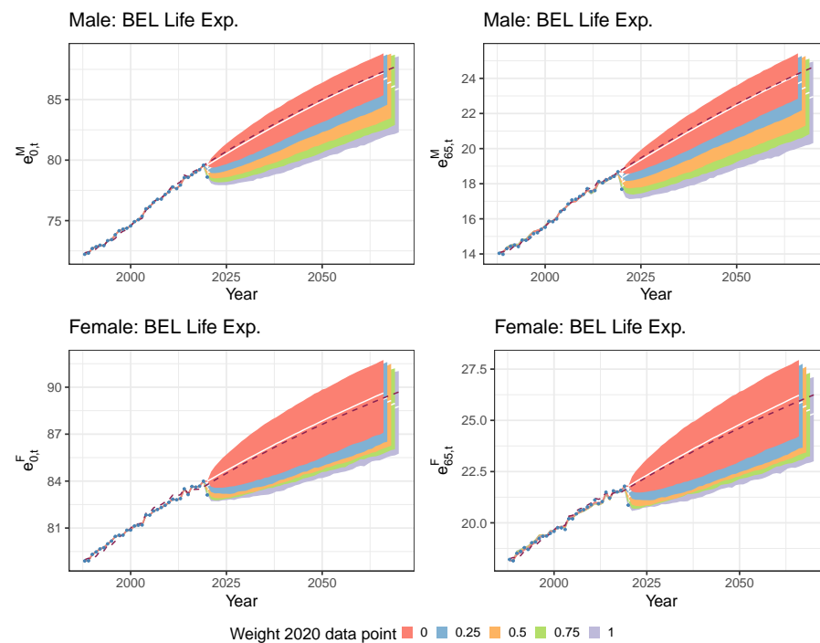
Figure 15. Estimated and projected period life expectancies \hat{e}_{x,t} for Belgium. Male (top) and female (bottom) data, ages 0 (left) and 65 (right), calibration period 1988–2020, projection period 2021–2070. Calibration and projection is based on the method in Section 5.1. We show the 0.5% quantile, median (white lines) and 99.5% quantile (fan charts), based on 10,000 simulations, across each weighting scenario. The dark red, dashed line shows the 50% quantile originating from the original IA|BE 2020 model. The blue dots represent the observed period life expectancies.
