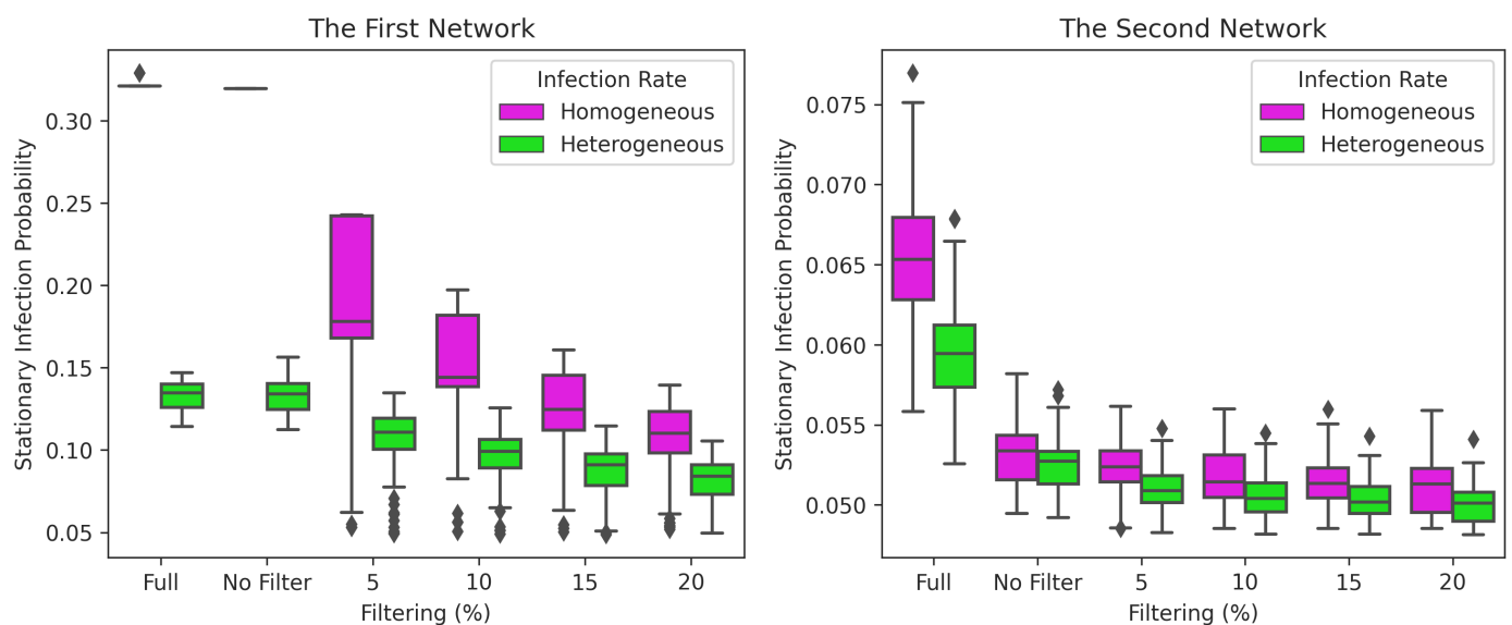
Figure 13. Stationary infection probabilities of nodes based on filters and infection rates in the first and second network. There are two cases for homogeneous and heterogeneous infection rates: (1) without GMA (Full), and (2) with GMA (using filter 0% (No Filter), 5%, 10%, 15% and 20%).
