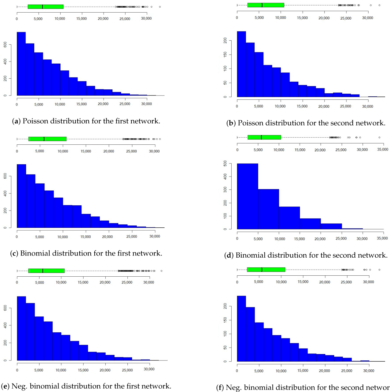
Figure 9. Distributions of the number of communication for one year contract using a link-based model.
