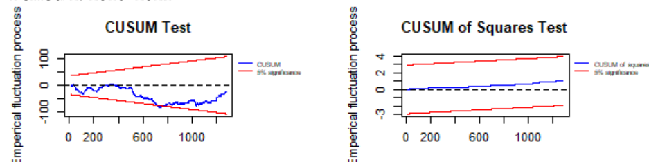
Figure 4. CUSUM and CUSUM of squares tests.
