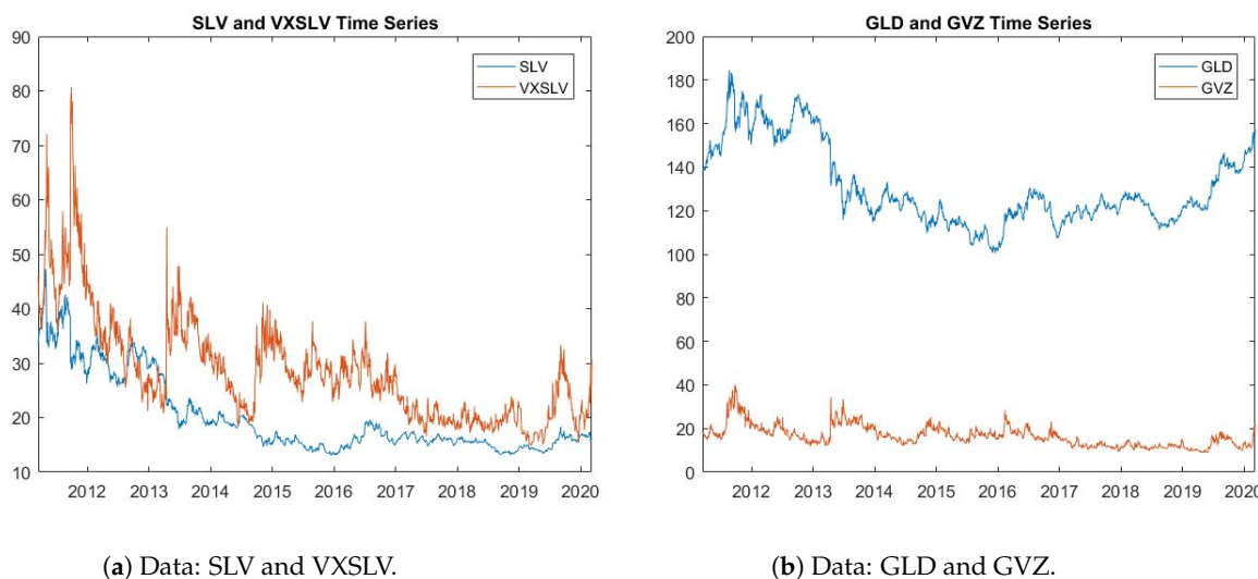
Figure 3. Historical SLV (VXSLV) and GLD (GVZ) data.
