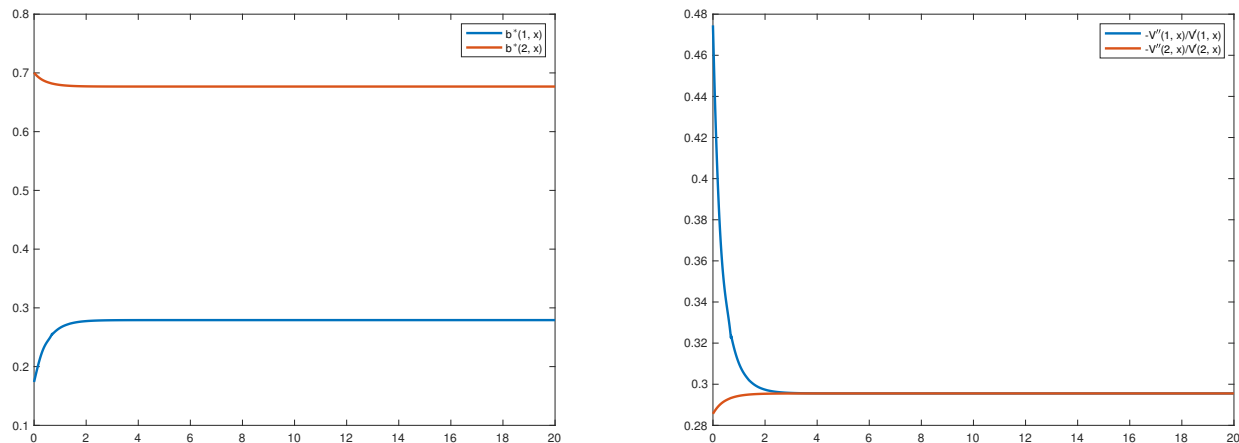
Figure 2. The optimal reinsurance strategies (left) and the ratios -V''/V' (right).
