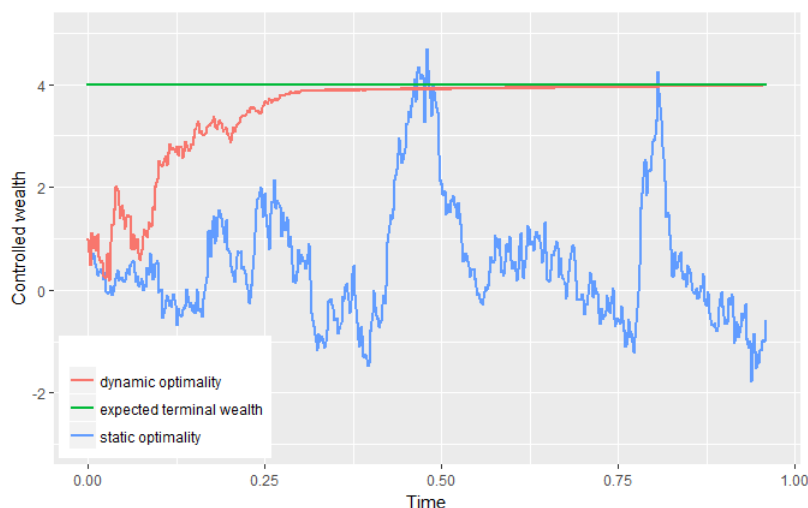
Figure 5. Statically optimal wealth X_t^s and dynamically optimal wealth X_t^{d*} .
