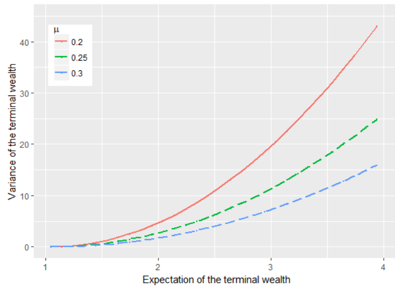
Figure 2. The impact of \mu on the efficient frontier.
