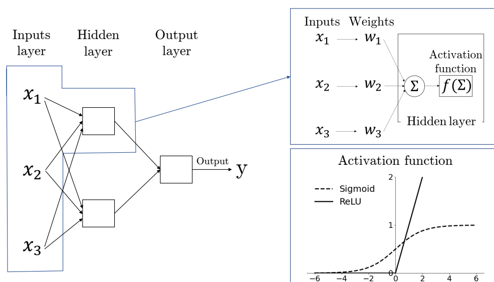
Figure 1. Architecture of a feedforward neural network.
