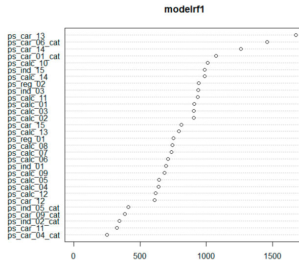
Figure 13. The rank of features by importance based on the random forest algorithm.
