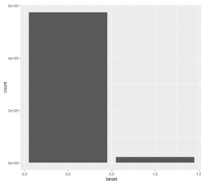
Figure 5. Histogram of the distribution of target values.
