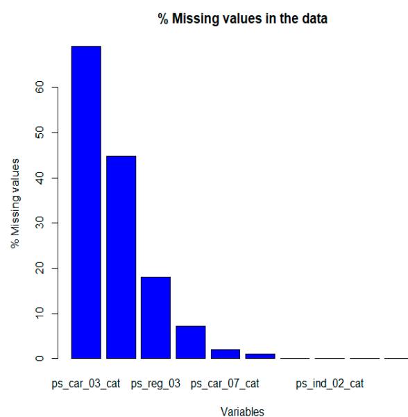
Figure 8. Missing values in our data.
