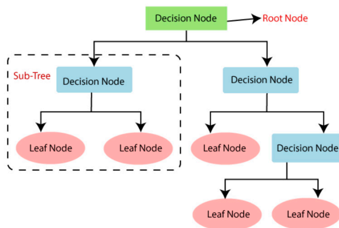
Figure 1. Structure of a general decision tree.
