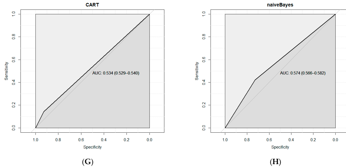
Figure 12. ROC and calculated AUC obtained for the classifier models of (A) RF, (B) C50, (C) XGBoost, (D) J48, (E) K-NN, (F) LR, (G) caret, and (H) naïve Bayes.
