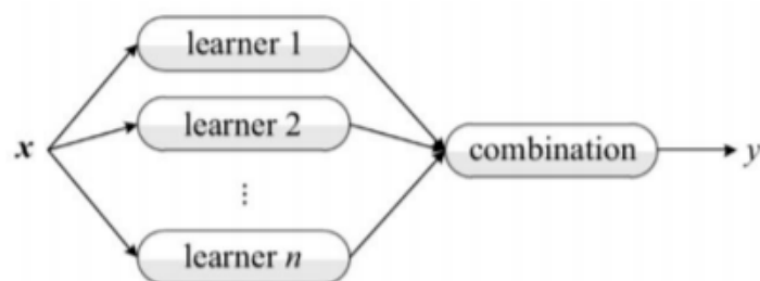
Figure 2. XGBoost methodology.
