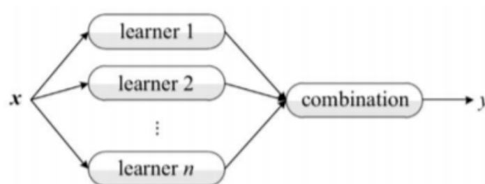
Figure 2. XGBoost methodology.
