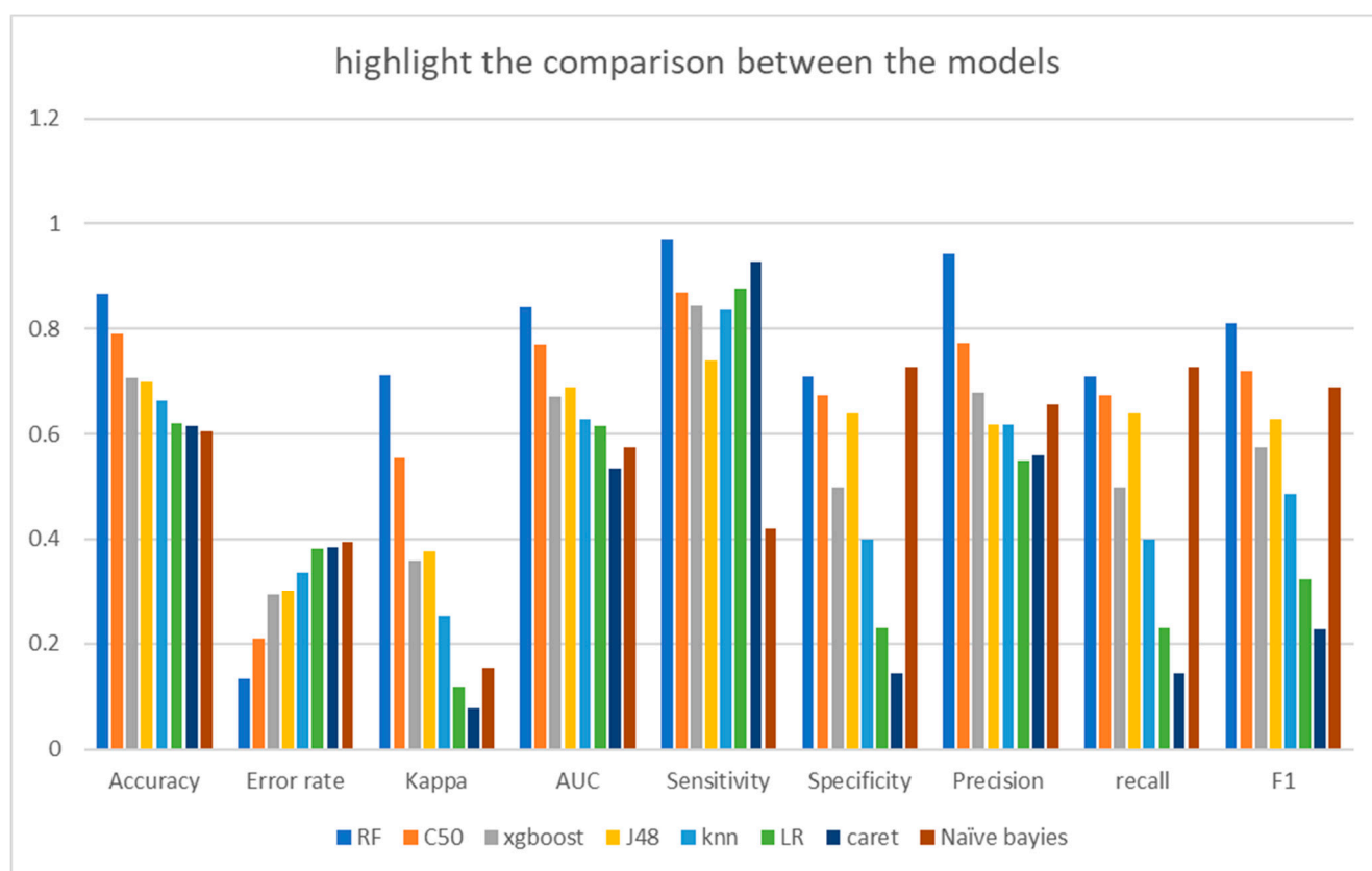
Figure 11. Comparison between the models.
