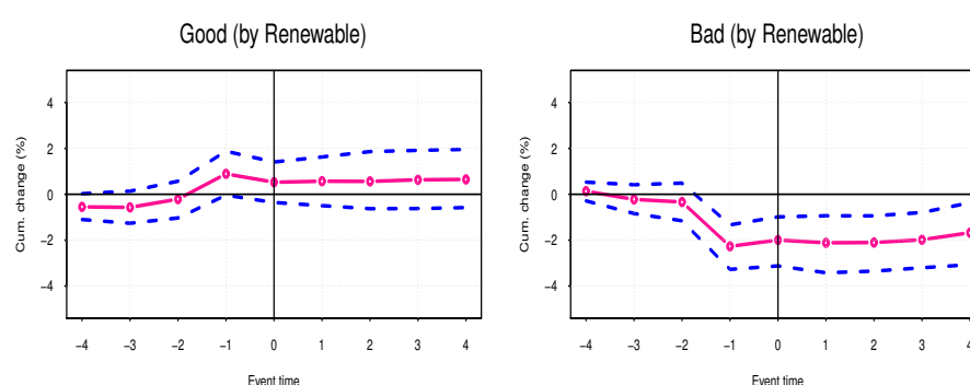
Figure 10. Extreme event on Renewable and response of WTI oil.
