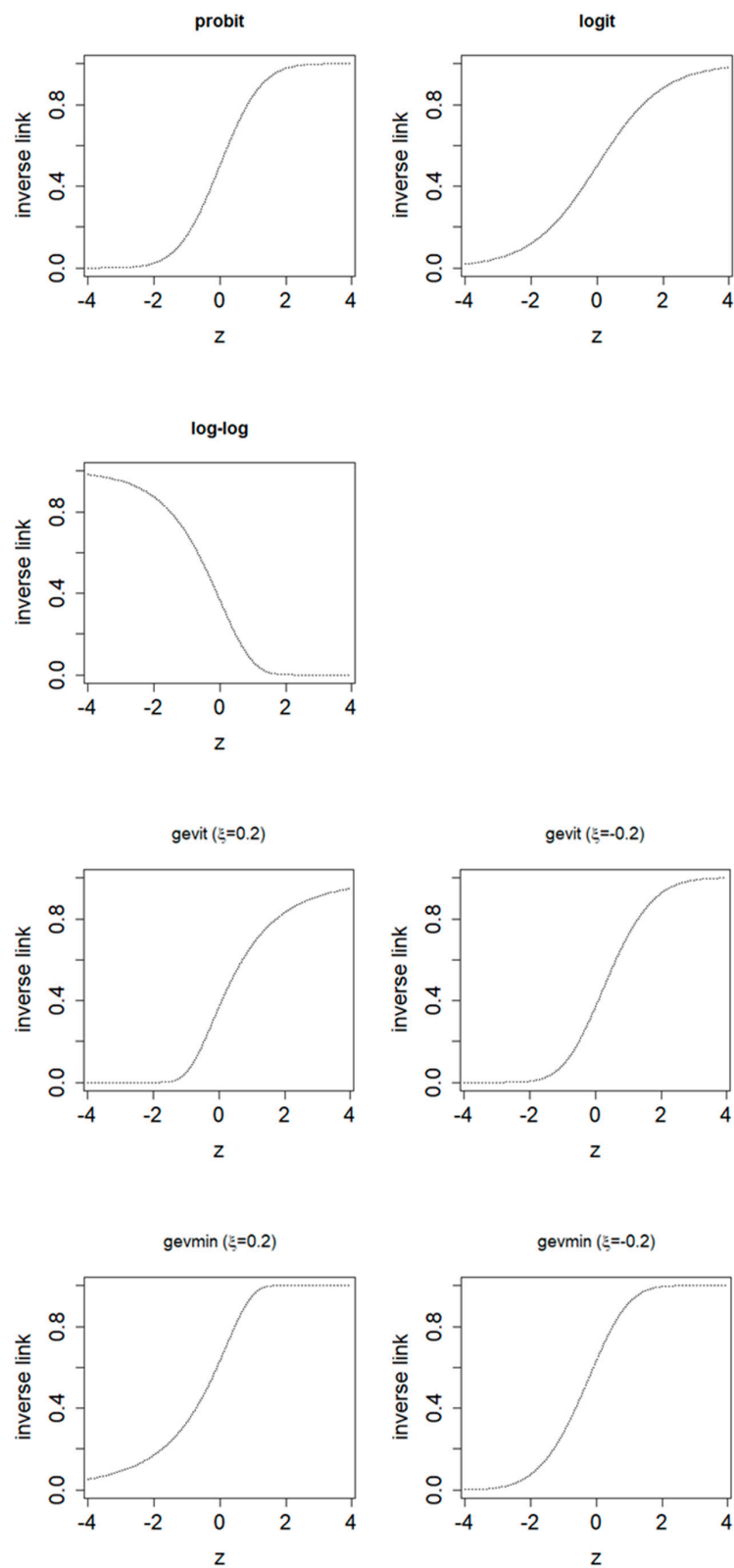
Figure 2. Five different (inverse) link functions.
