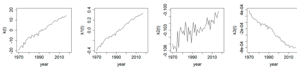
Figure 4. Trends of k_t and k_{t,1} to k_{t,3} based on five link functions for non-annualised survival probabilities of Australian females.
