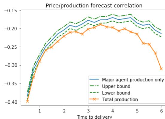
Figure 3. Correlation between the price increments and the major player renewable production increments vs. the correlation between the price increments and the total renewable production increments.
