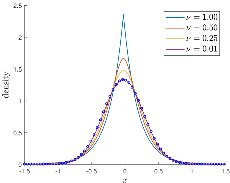
Figure 1. Black–Scholes (circles) as the limit of VG(\sigma, \nu, 0) \xrightarrow{\nu \rightarrow 0} BS(\sigma) .
