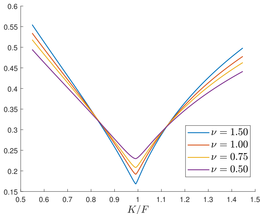
Figure 4. Implied volatility smiles of VG( \sigma, \nu, 0 ) obtained by Formula (1). Params: \sigma = 0.3, \tau = 0.2, r = 1\%, q = 0\%, S_t = 4000 . The moneyness is determined by F := S_t \exp((r - q)\tau) .
