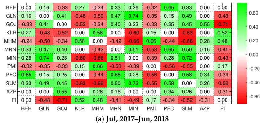
Figure A2. Extreme downside hedging (EDH) matrix for different \tau values.
