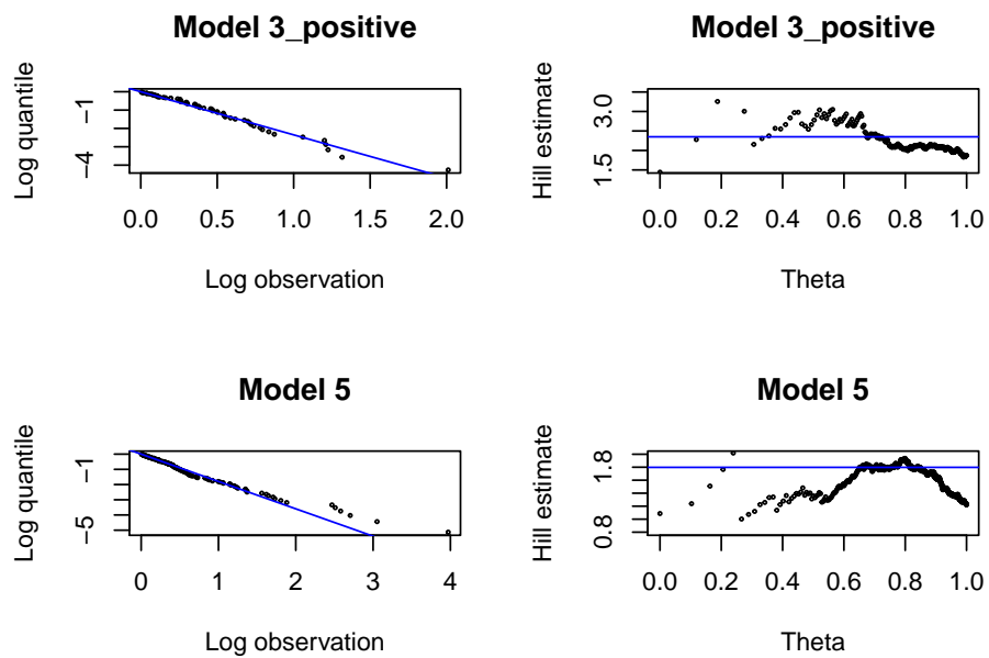
Figure A5. Pareto quantile plots and alHill plots for incremental payments and changes in claim incurred in k = 8 .
