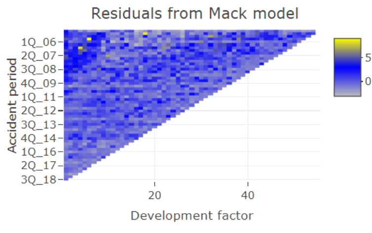
Figure A19. Residuals from Mack model fitted to development factors in a run-off triangle.
