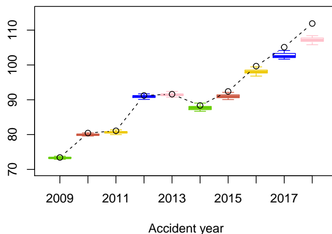
Figure 2. Boxplots of the aggregate ultimate payments from the RBNS claims (in MM). The dots indicate the Chain-Ladder estimates.
