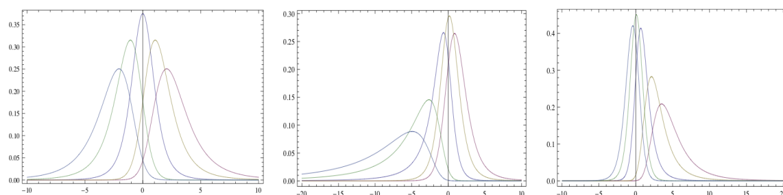
Figure 1. Graphics of the probability density function: left for the skewed t_1 (1) when (a, b) = (2, 2) , (5, 2) , (8, 2) , (2, 5) , and (2, 8) ; center for the skewed t_2 (2) with (a, b, c) = (2, 2, 0.5) , (8, 2, 0.5) , (5, 2, 0.5) , (2, 5, 0.5) , and (2, 8, 0.5) ; and on the right, (2, 2, 2) , (8, 2, 2) , (5, 2, 2) , (2, 5, 2) , and (2, 8, 2) .
