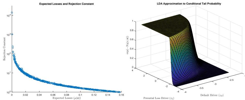
Figure 1. The left panel of this figure illustrates the relationship between expected losses \mu(z) and the second-stage rejection constant \hat{c} = \hat{c}(x, z) , in the two-factor model. The right panel illustrates the graph of the LDA approximation of Equation (13). Parameters (randomly selected using the procedure in Section 5.3) in both panels are (P, \rho_D, \rho_L, \rho_I, \rho_S, a, b, N) = (0.0063, 0.3964, 0.2794, -0.3356, -0.7599, 0.6497, 0.5033, 134) and the threshold is x = 0.1575 . Mean losses are \mathbb{E}[L_i] = 0.0029 , and the probability that losses exceed the threshold x is on the order of 50 basis points. Points in the left panel were obtained by generating 1000 realizations of the systematic risk factors from their actual distribution (as opposed to the first-stage IS distribution) using the indicated parameter values.
