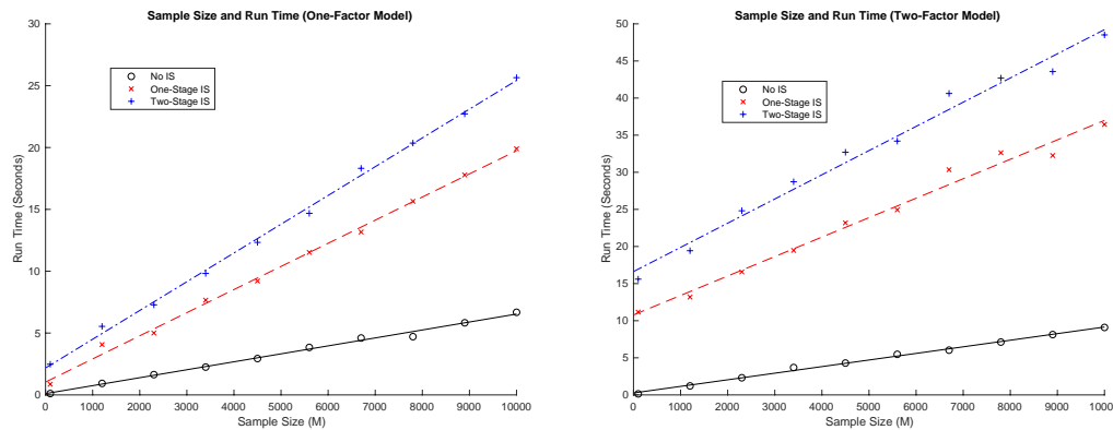
Figure 7. This figure illustrates the relationship between sample size ( M ) and run time (total CPU time required to estimate p_x by a particular algorithm), using a set of parameters randomly selected according to the procedure described in Section 5.3. For each value of M we use a pilot sample that is 10% as large as the sample that is eventually used to estimate p_x (i.e., we set M_p = 0.1M ). The left panel corresponds to the one-factor model and parameter values are (P, \rho_D, \rho_L, \rho_I, \rho_S, a, b) = (0.0827, 0.1000, 0.3629, -0.0180, -1, 0.6676, 0.8751) and N = 2334 . The right panel corresponds to the two-factor model and parameter values are (P, \rho_D, \rho_L, \rho_I, \rho_S, a, b) = (0.0241, 0.2322, 0.0343, 0.1650, 0.4135, 0.4056, 0.4942) and N = 3278 .
