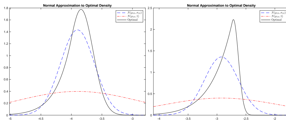
Figure 2. This figure illustrates f_x (in fact, the approximation of Equation (40)) for two randomly generated sets of parameters. Each panel superimposes (i) a normal density with the same mean and variance as f_x (dashed blue line), and (ii) a normal density with the same mean as f_x and unit variance (dash-dot red line). The mean and variance of f_x are computed via (computationally inefficient) quadrature. The mean and variance of f_x are computed using quadrature. Parameters in the right panel are (P, \rho_D, \rho_L, \rho_I, \rho_S, a, b, N) = (0.02, 0.33, 0.27, 0.96, 1, 2.47, 4.32, 454) , and for the left panel they are (P, \rho_D, \rho_L, \rho_I, \rho_S, a, b, N) = (0.03, 0.13, 0.12, 0.85, 1, 1.81, 1.90, 271) . In both cases, the transformation h is taken to be h(x) = B_{a,b}^{-1}(\Phi(x)) .
