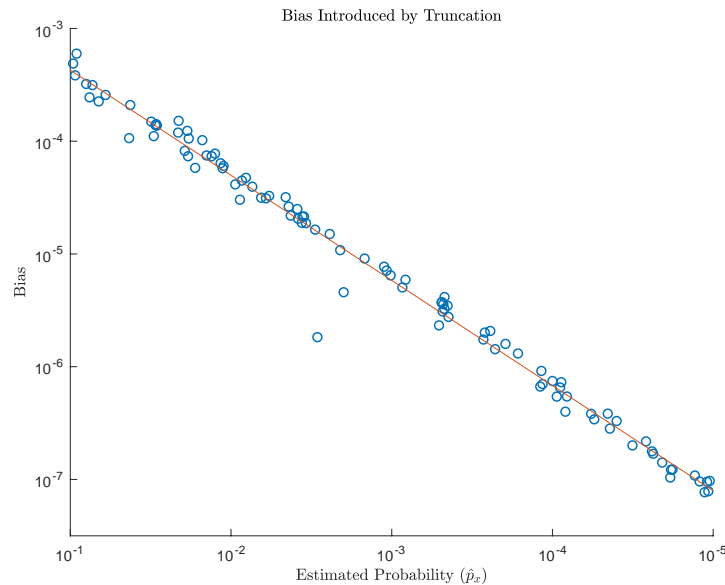
Figure 4. This figure illustrates the bias introduced by trimming large weights (vertical axis) as a function of the probability of interest (horizontal axis), for 100 randomly generated parameter sets in the one-factor case. For each set, we compute bias (in fact, an upper bound on the bias) by using quadrature to approximate Equation (46) and estimate the probability of interest using the full two-stage algorithm.
