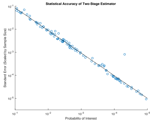
Figure 6. This figure illustrates the relationship between \nu_x and p_x , where \nu_x is the standard deviation of \Lambda_1(\mathbf{Z})\Lambda_2(\bar{L}_N, \mathbf{Z})\mathbf{1}_{\{\bar{L}_N \geq x\}} under the two-stage IS density of Equation (32), in the two-factor case. The numerical values of p_x and \nu_x are estimated for each of 100 randomly generated parameters sets, according to the procedure described in Section 5.3.
