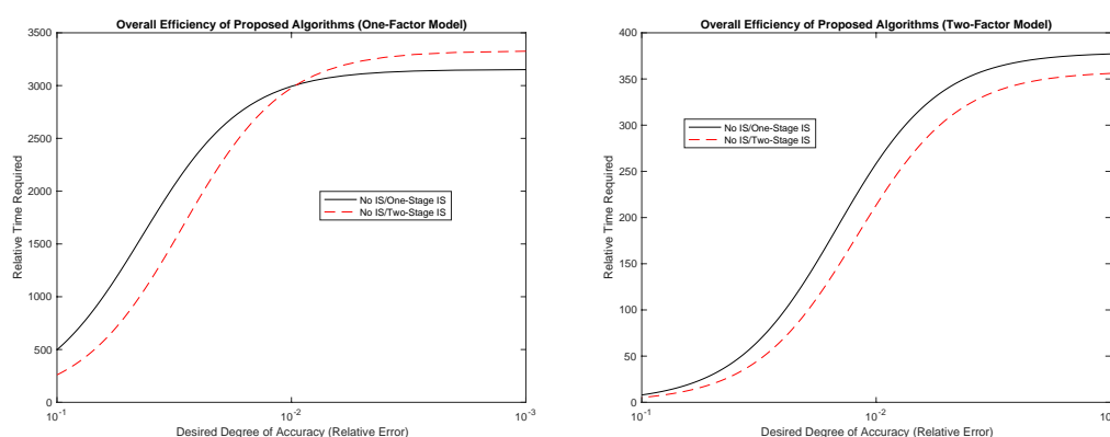
Figure 8. This figure illustrates the overall efficiency of the proposed algorithms. Specifically, the solid [dashed] line in the left panel illustrates the ratio of (i) the total run time (in seconds) required to ensure that the standard estimate's relative error does not exceed a given threshold to (ii) the run time required by the one-stage [two-stage] algorithm, in the one-factor model. The right panel corresponds to the two-factor model. Parameter values are the same as in Figure 7 and Table 3.
