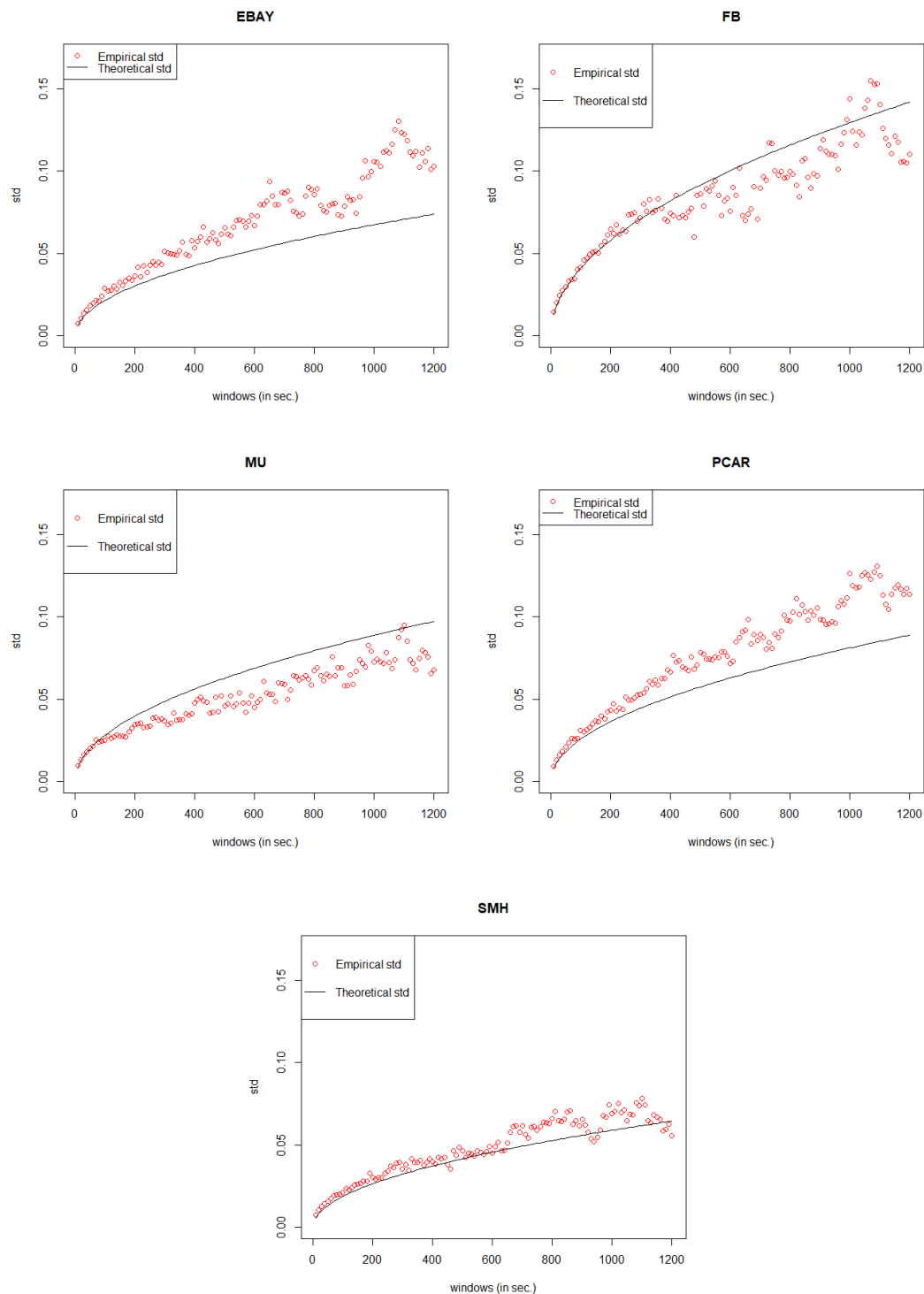
Figure 6. General Compound Hawkes Process with 2 non-fixed Dependent Oorder model fitting results.
