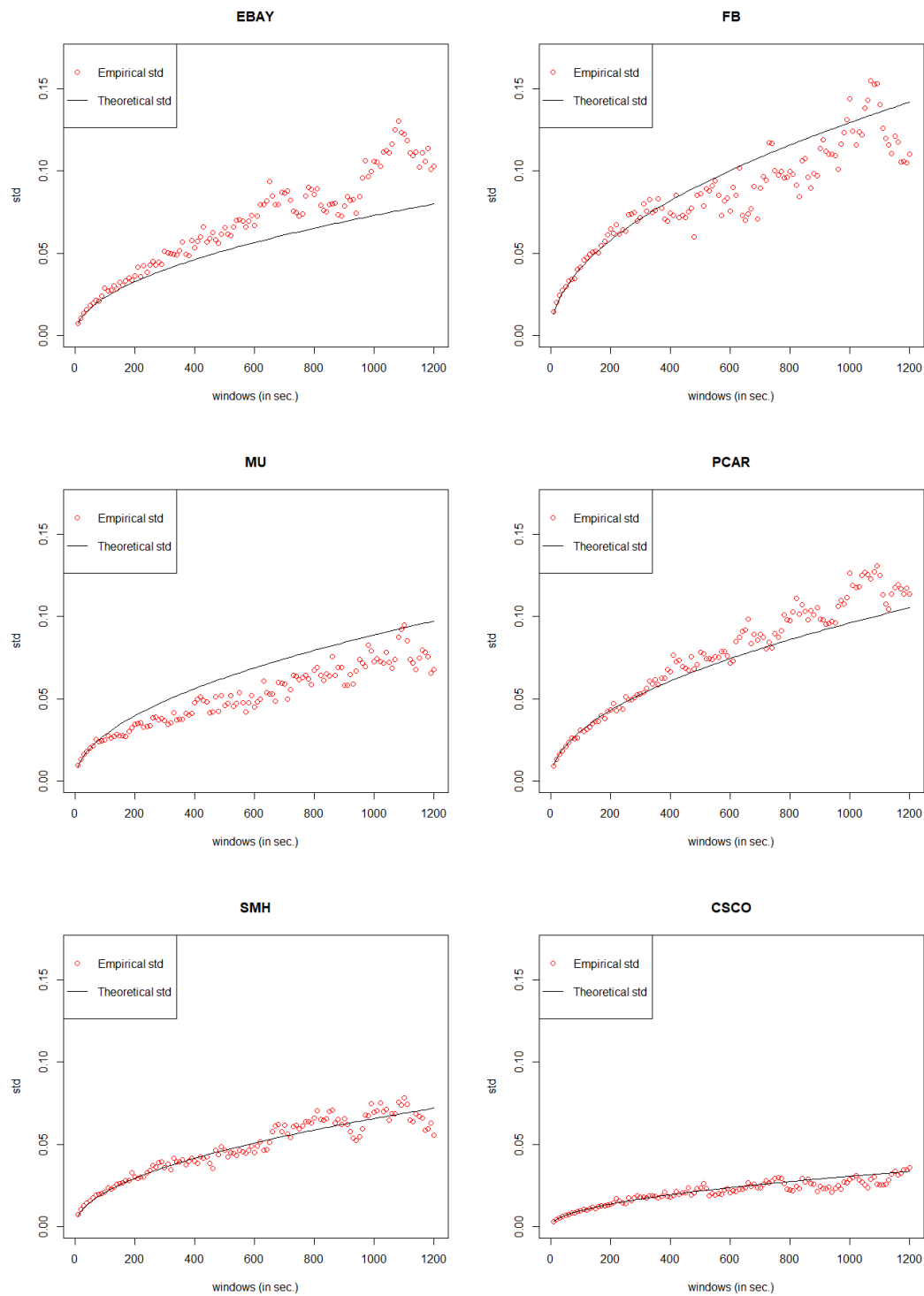
Figure 7. Best model fitting results for 6 stocks.
