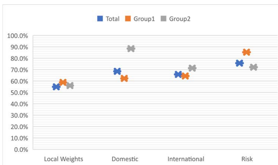
Figure 13. Consensus measure.
