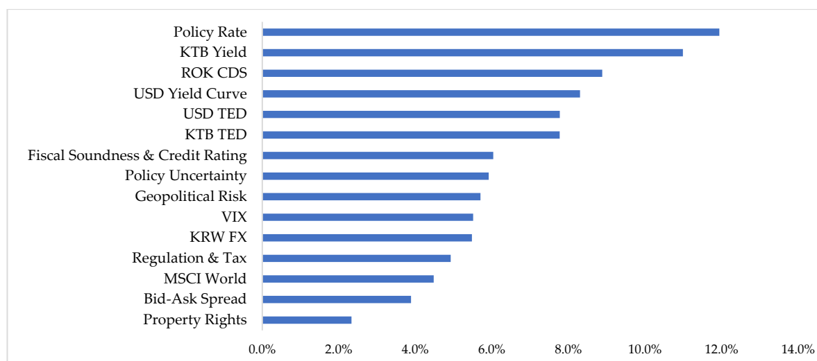
Figure 7. Global weights.
