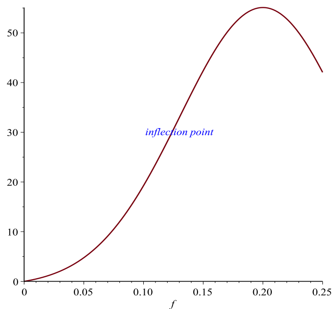
Figure 2. Inflection point.
