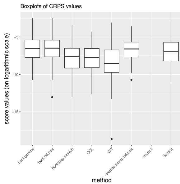
Figure 4. Boxplots of CRPS values from the commercial auto data.
