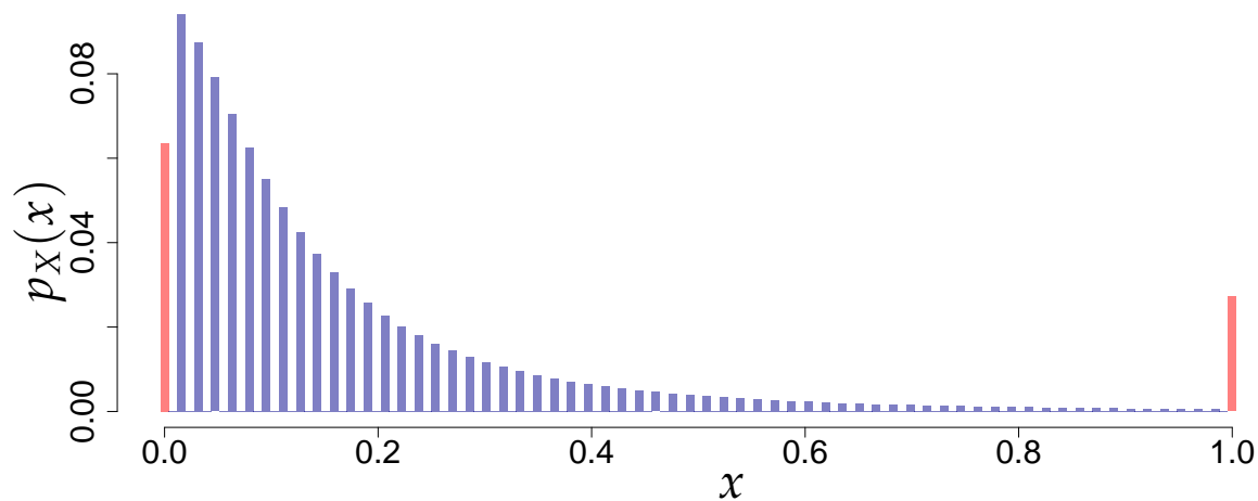
Figure 3. A discrete loss pdf represented as a mixture of two “spikes” (atoms) at minimum and maximum x damage ratio (red) and the main part (blue). Damage ratio is discretized on 64-point grid.
