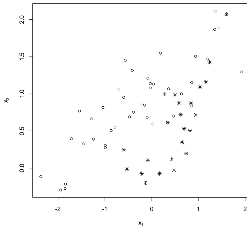
Figure 2. Hypothetical development data (circles) and review data (stars) for two explanatory variables x_1 and x_2 .
