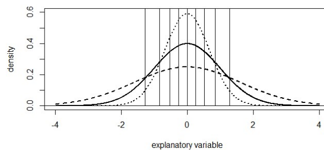
Figure 1. Distribution of continuous explanatory variable used to generate the development (solid line) and review data for example 1 (dashed line) and example 2 (dotted line). Boundaries of categories 1 to 10 are defined by the vertical lines, dividing the scale into 10 intervals each with 10% of the development data.
