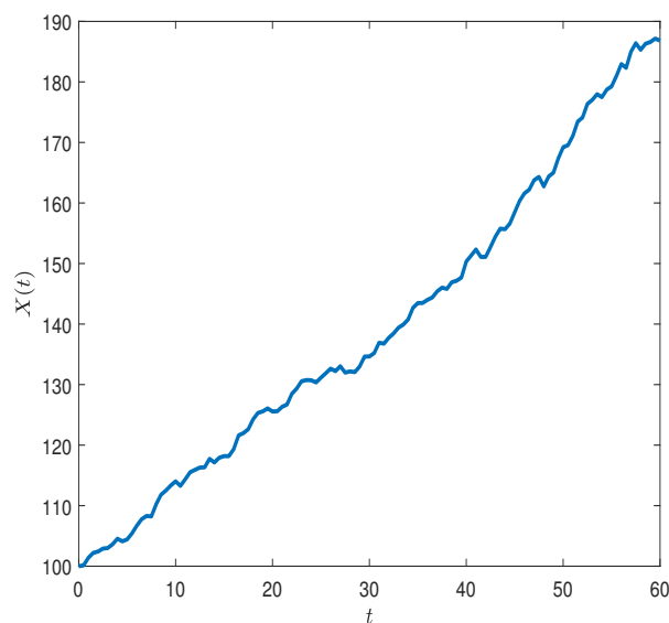
Figure 1. Wealth X(t) as a function of t .
