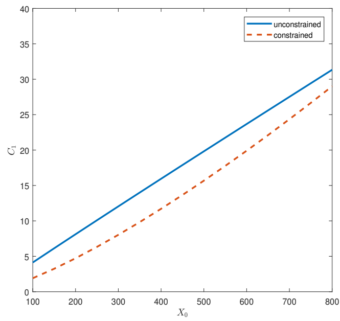
Figure 7. Optimal consumption C at time 1 as a function of initial wealth X_0 .
