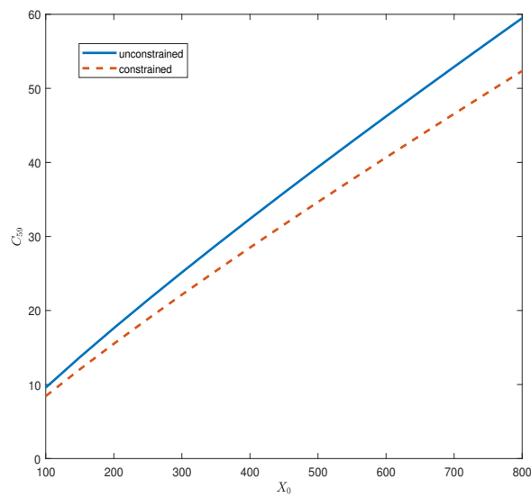
Figure 8. Optimal consumption C at time 59 as a function of initial wealth X_0 .
