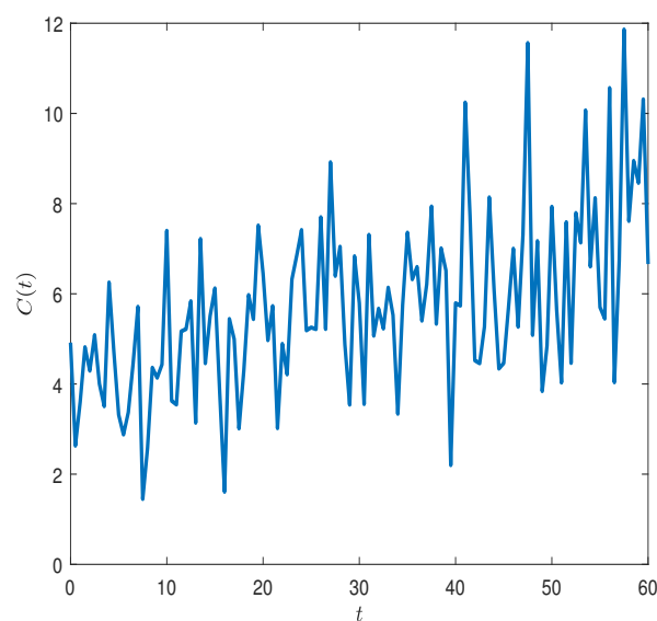
Figure 2. Optimal consumption C(t) as a function of t .
