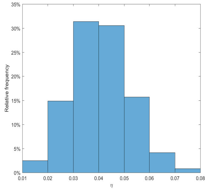
Figure 4. Relative frequency of consumption.
