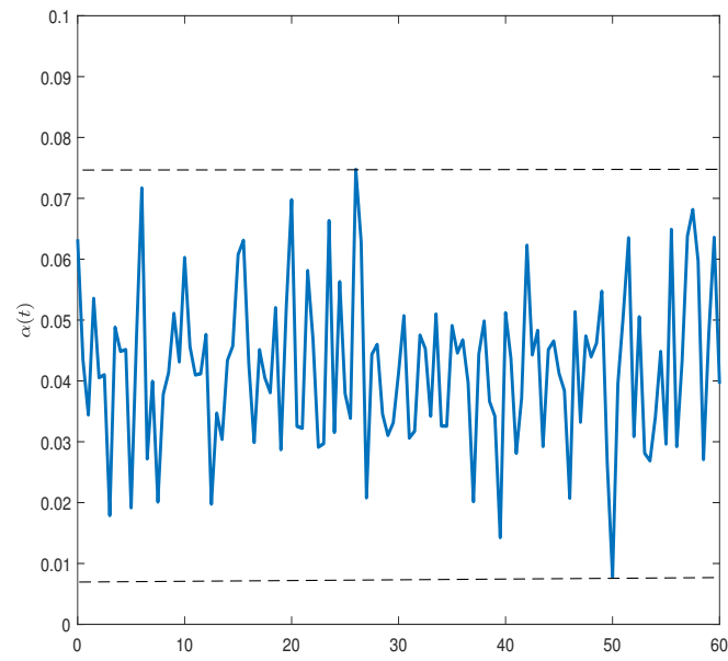
Figure 6. Optimal attention \alpha(t) as a function of t .
