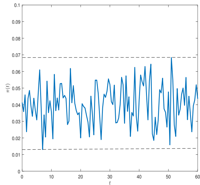
Figure 5. Optimal proportion of risky assets \pi(t) as a function of t .
