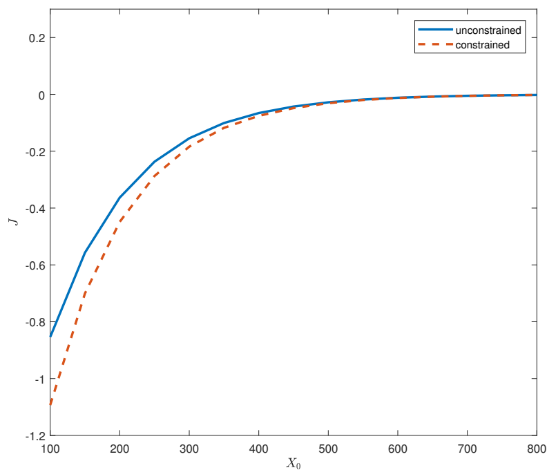
Figure 9. Value function J as a function of initial wealth X_0 .
