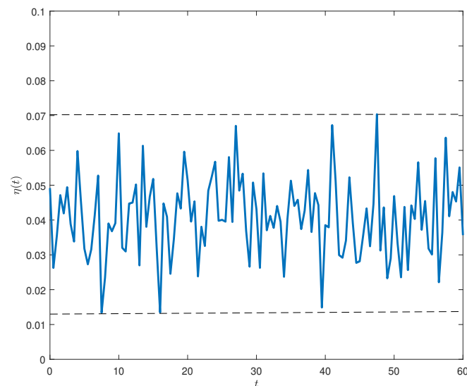
Figure 3. Optimal proportion of consumption \eta(t) as a function of t .
